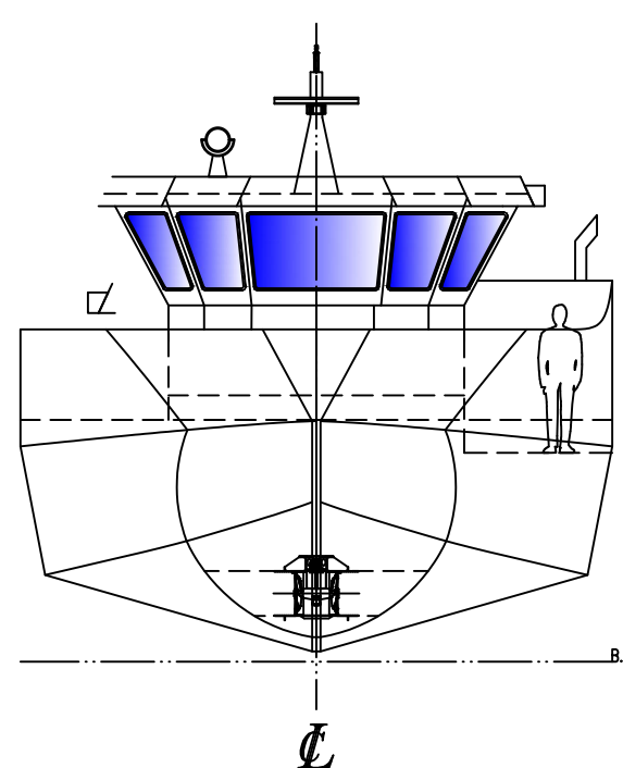
FORESHIP – LOOKING AFT
