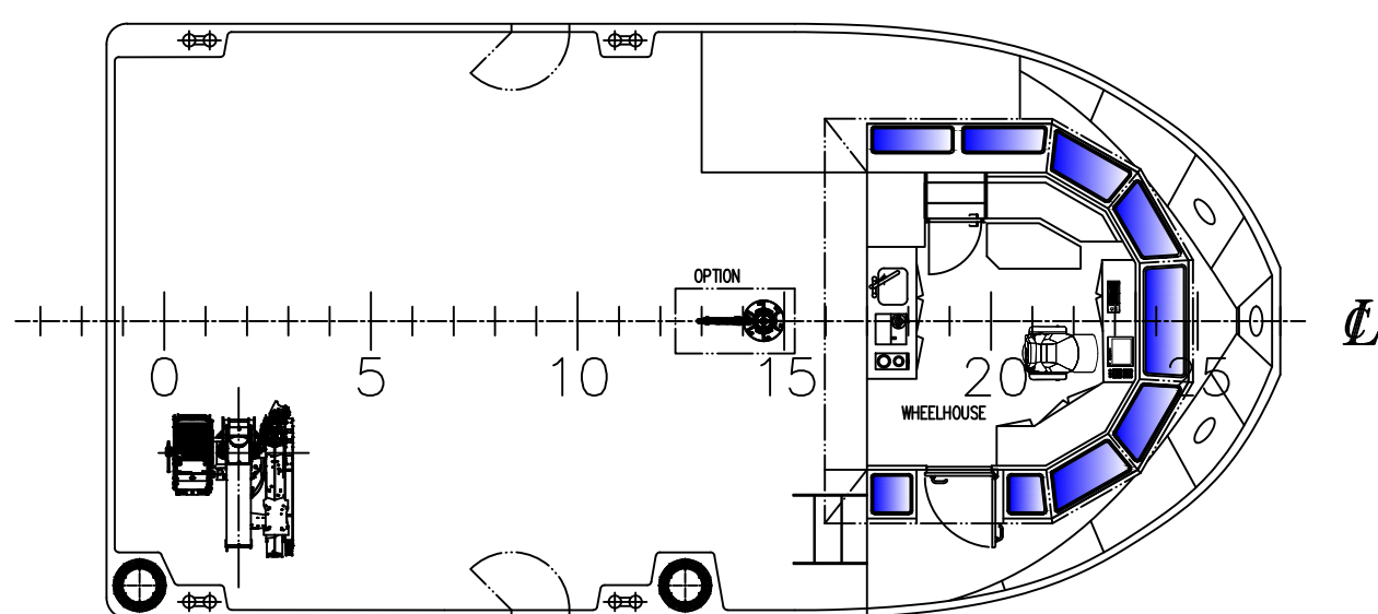
WHEELHOUSE DECK
