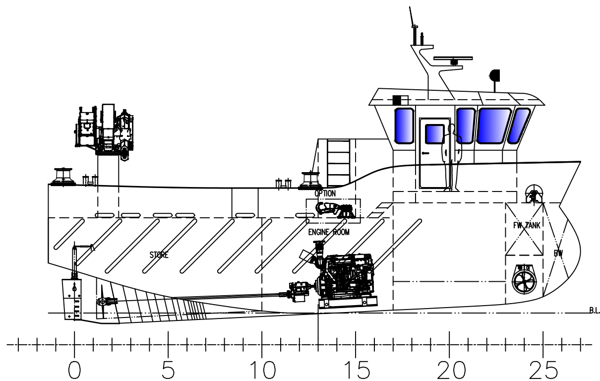
PROFILE VIEW (SB)
