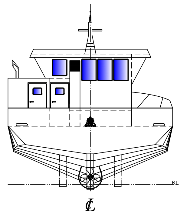
AFTSHIP – LOOKING FORWARD
