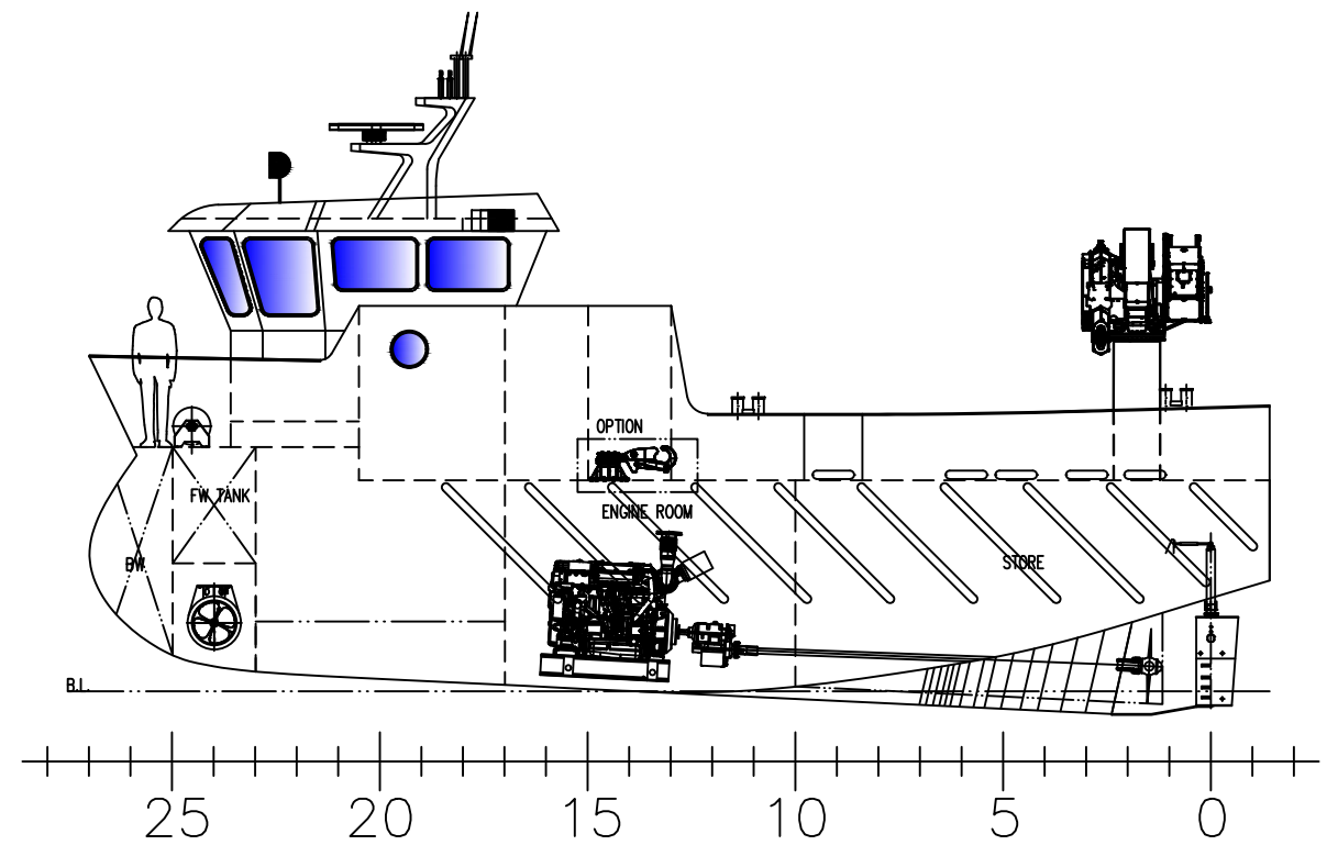
PROFILE VIEW (PS)
