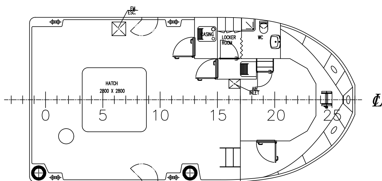
MAIN DECK
