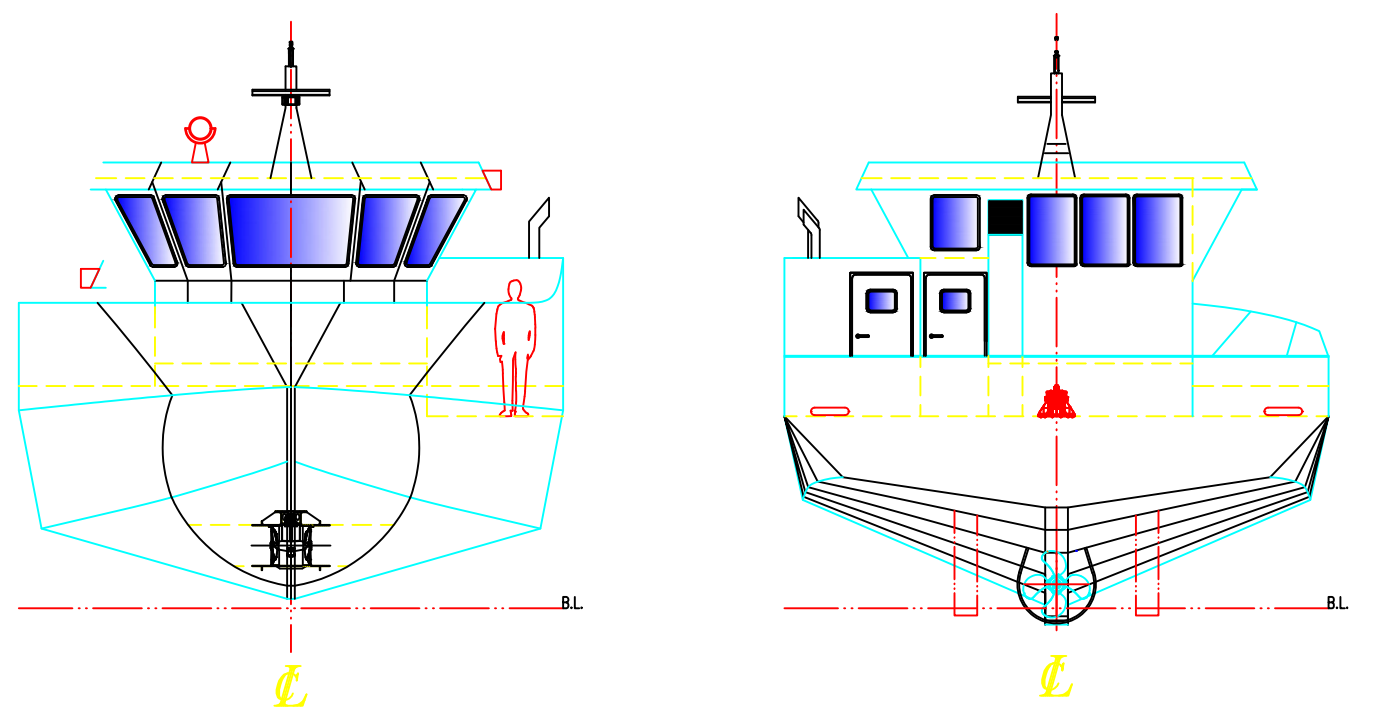
FORESHIP – LOOKING AFT
